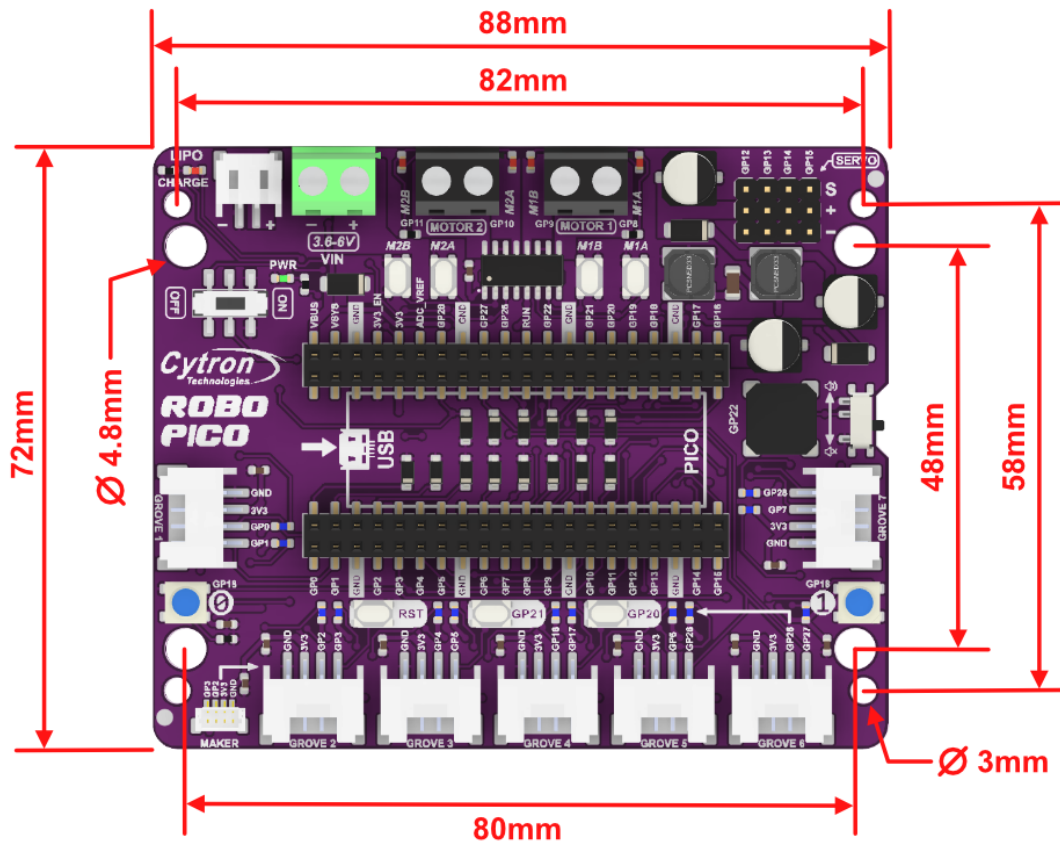
Figure 4: ROBO-PICO Dimension
