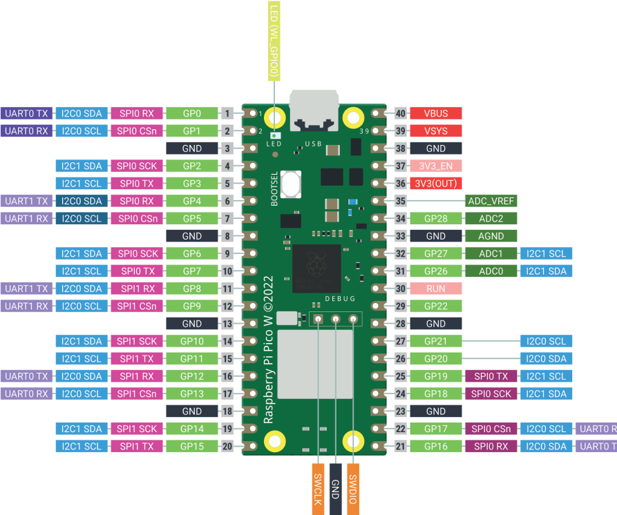
Figure 3: Raspberry Pi Pico W Pinout Diagram
